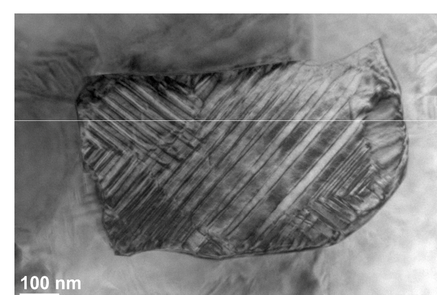
Domain structure in \text{Na}_{0.4}\text{K}_{0.1}\text{Bi}_{0.5}\text{TiO}_3 ceramics
